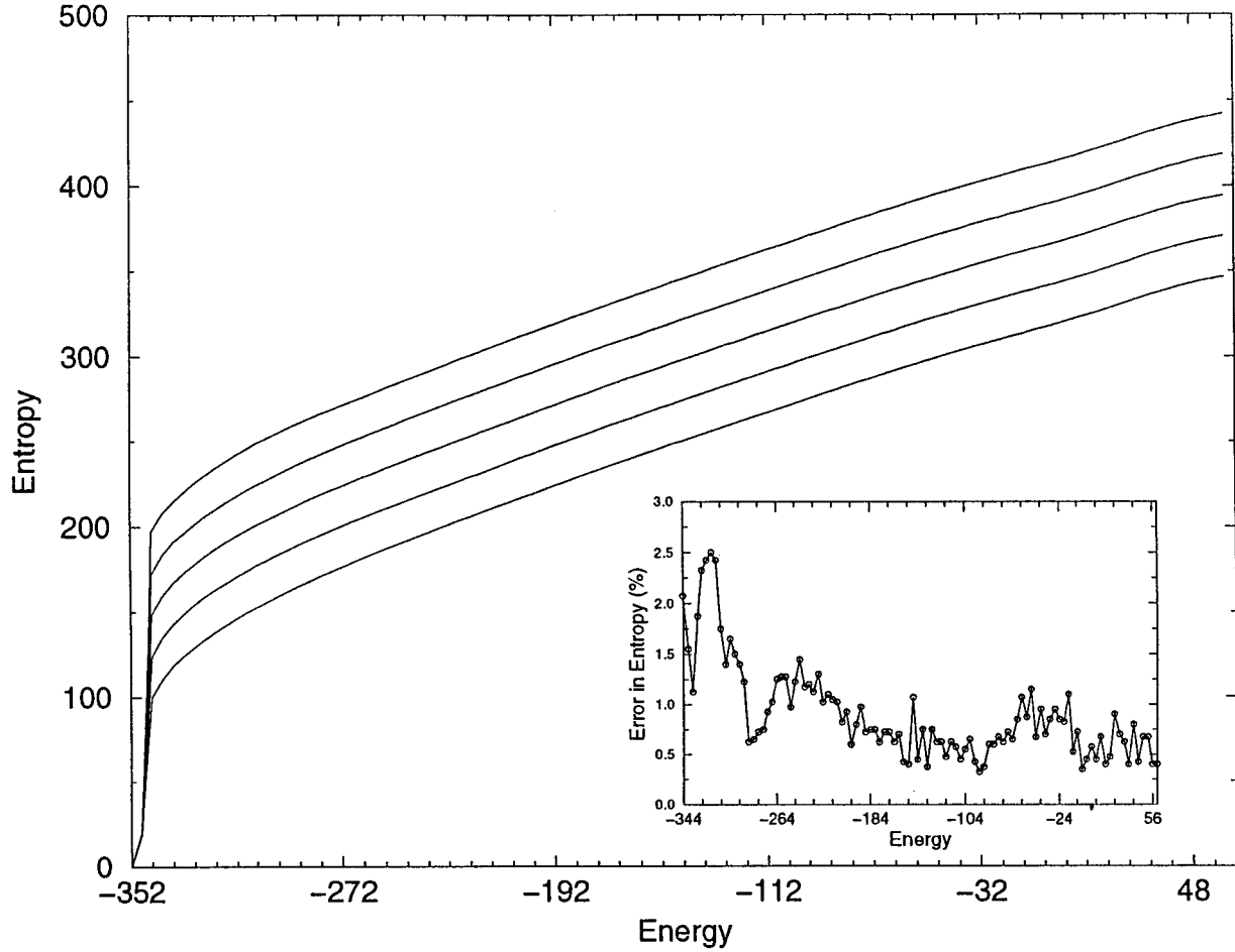
FIGURE 2 Entropy of the dimer of GCN4-lz as a function of its energy. The five different entropy curves have been obtained from last five successive iterations of the ESMC run after convergence of the simulations. The inset shows the error in entropy plotted as a function of the energy.
