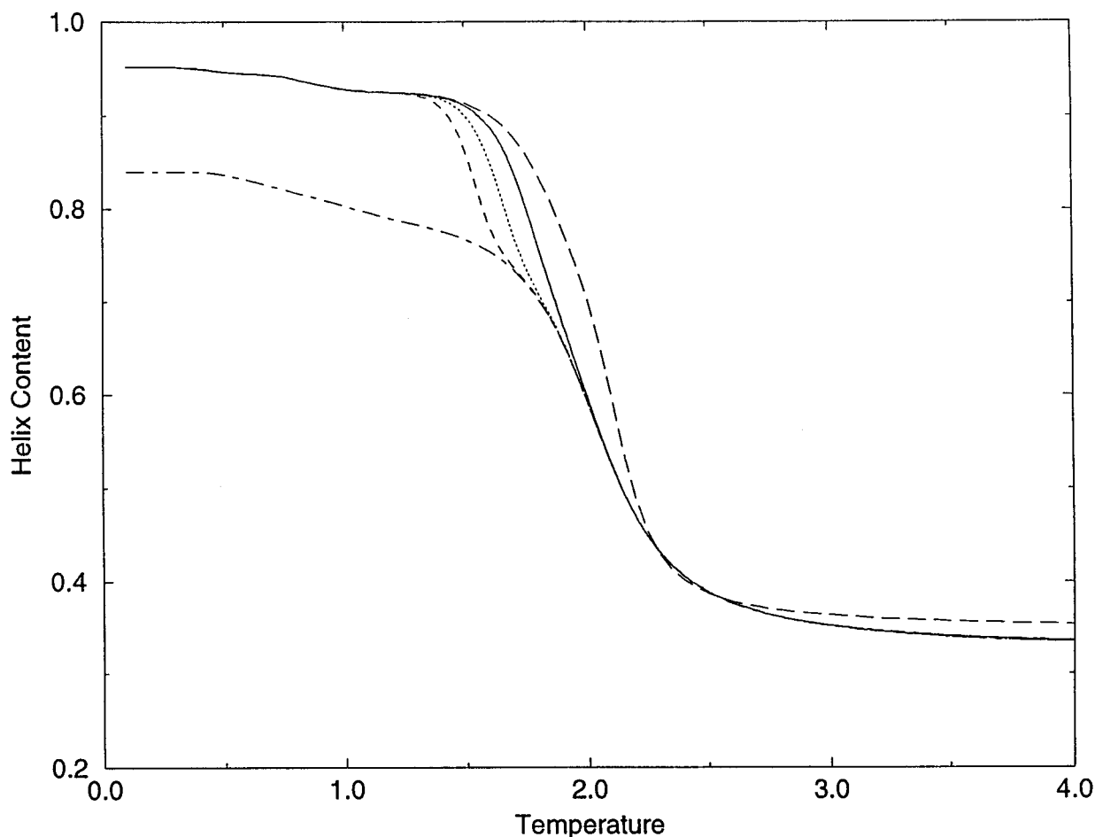
FIGURE 1 The average helix content versus temperature curves for simulations with parameter set I. The dashed and dashed-dotted lines represent the average helix contents of the dimer and monomer, respectively. The dashed, dotted, and solid lines represent the overall helix contents at chain concentrations of 2 \mu\text{M} , 43 \mu\text{M} , and 1 mM, respectively.
